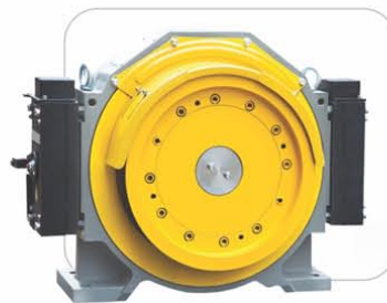
Gearless Machine
