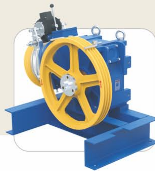
High Speed Traction M/c.
